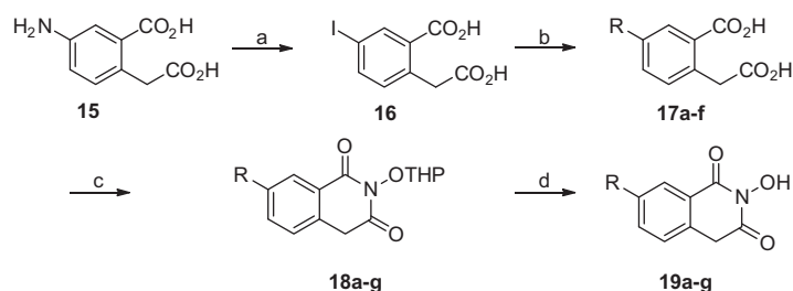
Scheme 1. Synthesis of C-7 substituted 2-hydroxyisoquinoline-1,3-diones. Reagents and conditions: (a) 4 N aq sulfuric acid, NaNO 2 , –10 °C, then urea, –10 to 0 °C, KI, rt overnight, 44%; (b) boronic acid, Pd(PPh 3 ) 4 , K 2 CO 3 , H 2 O: EtOH (v/v = 1:1), microwave, 150 °C, 30 min, 87%-quant; (c) THPONH 2 , ClPh, CDI, reflux 30 s; (d) p -TSA hydrate, MeOH, 6–22% over two steps.
