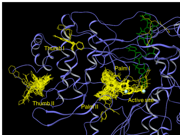
Figure 3. Binding sites of HCV NS5B inhibitors.
