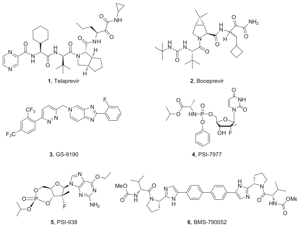
Figure 1. Representative HCV inhibitors: 1 and 2 , protease inhibitors; 3 , nonnucleoside polymerase inhibitor; 4 and 5 , nucleoside polymerase inhibitors; 6 , NS5A inhibitor.
