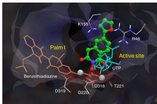
Figure 4. Docking of 27a (green) in HCV NS5B polymerase active site. The chelation of both Mg 2+ ions (light blue sphere) allows the placement of the C-6 furan ring in close proximity to R48 and K155, allowing the formation key H-bond for potent inhibition. Both UTP (cyan) (taken from PDB: 1NB6 45 ) and benzothiadiazine (brown) (taken from PDB:3HHK 46 ) are shown to highlight the unique mode of binding of compound 27a .
