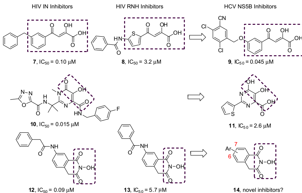
Figure 2. Design of novel NS5B inhibitor scaffold 14 based on the pharmacophore resemblance among HIV IN inhibitors, HIV RNH inhibitors and HCV NS5B inhibitors.
