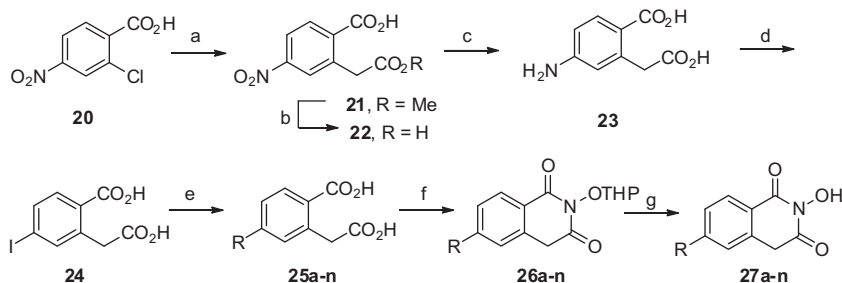
Scheme 2. Synthesis of C-6 substituted 2-hydroxyisoquinoline-1,3-diones. Reagents and conditions: (a) dimethyl malonate, CuBr, NaOMe, 92%; (b) NaOH, MeOH, rt overnight, 49%; (c) 10% Pd/C, H 2 , EtOH, 85%; (d) 4 N aq sulfuric acid, NaNO 2 , –10 °C, then urea, –10 to 0 °C, KI, rt overnight, 58%; (e) boronic acid, Pd(PPh 3 ) 4 , K 2 CO 3 , H 2 O: EtOH (v/v = 1:1), microwave, 150 °C, 30 min, 59%-quant; (f) THPONH 2 , ClPh, CDI, reflux 30 s; (g) p -TSA hydrate, MeOH, 10–24% over two steps.
